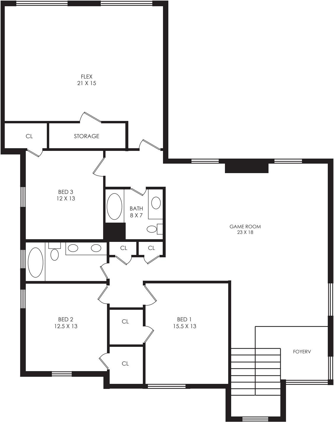
SECOND FLOOR 2060 SQ FT
